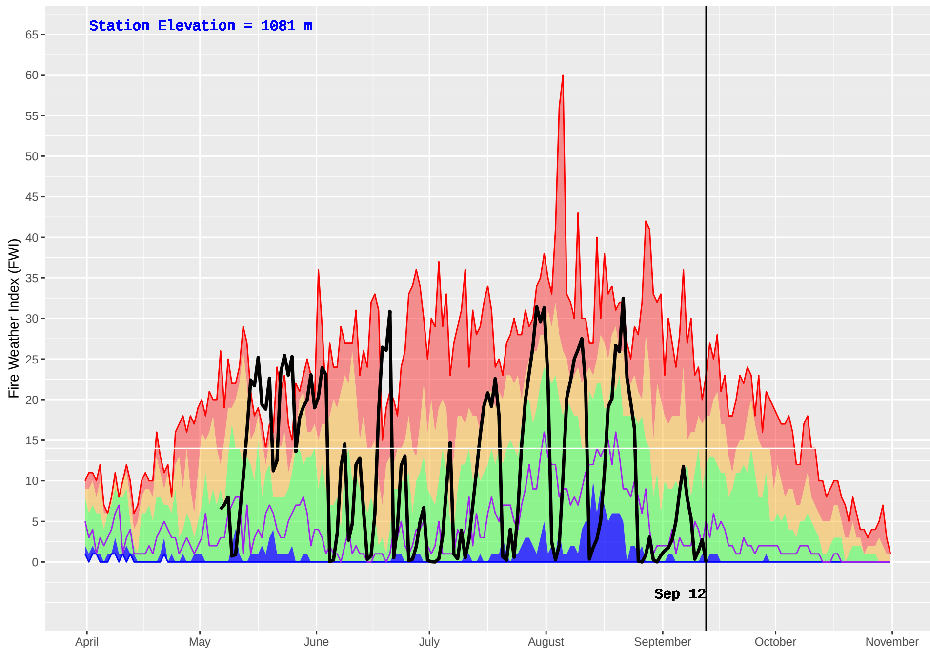
GAVIN (227) : Historical (1981–2016) and Current (2018) Daily Fire Weather Index (FWI)
