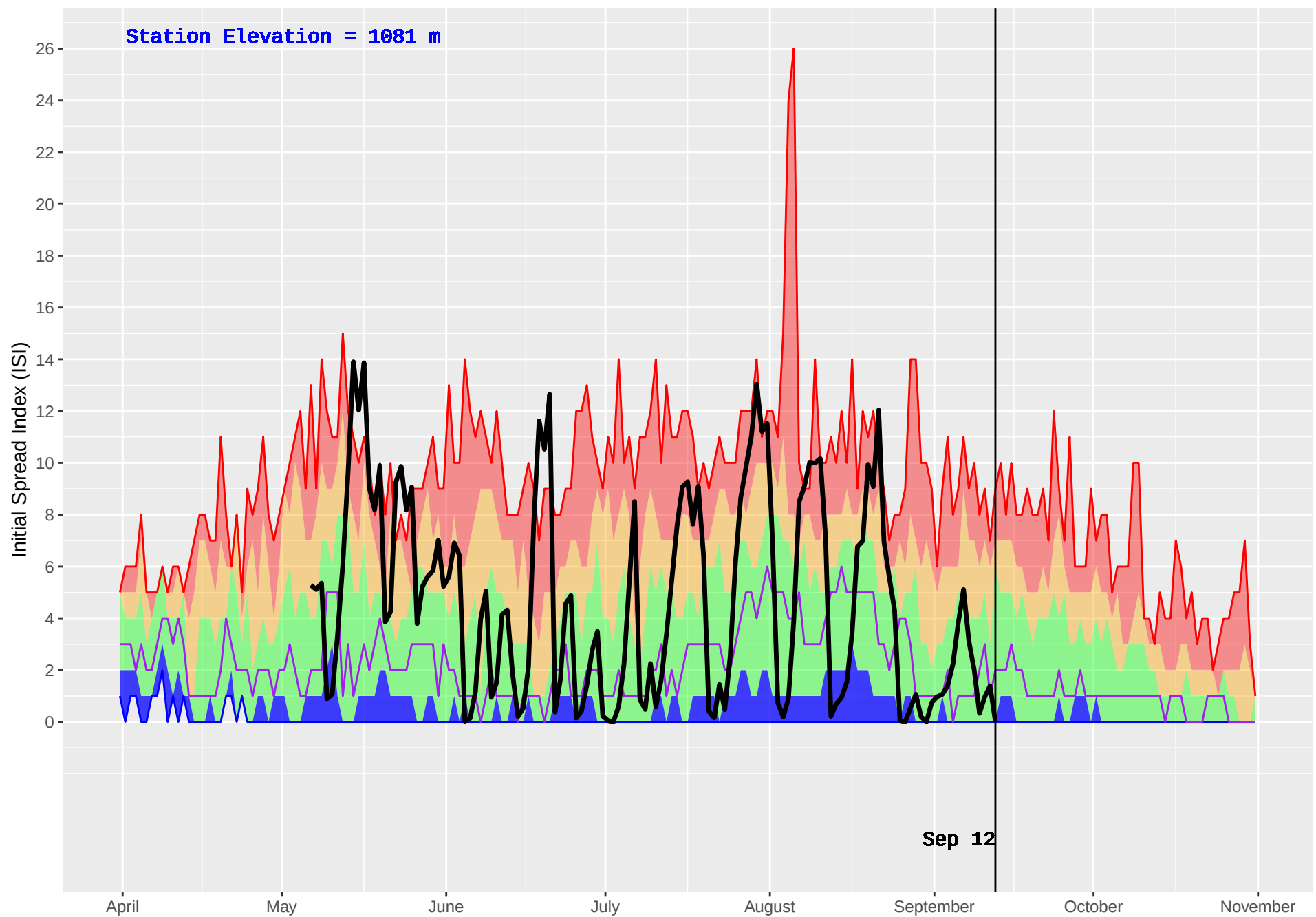
GAVIN (227) : Historical (1981–2016) and Current (2018) Daily Initial Spread Index (ISI)
